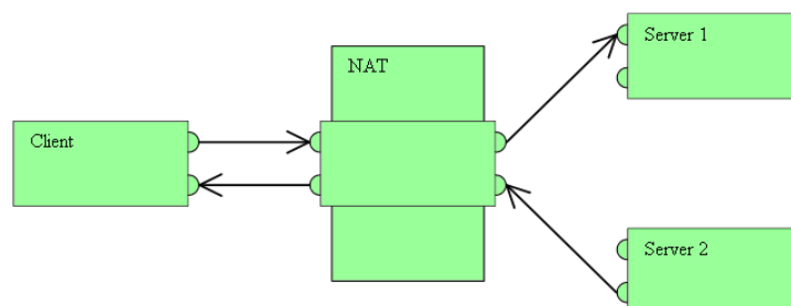
Figure 1 - Full Cone NAT
