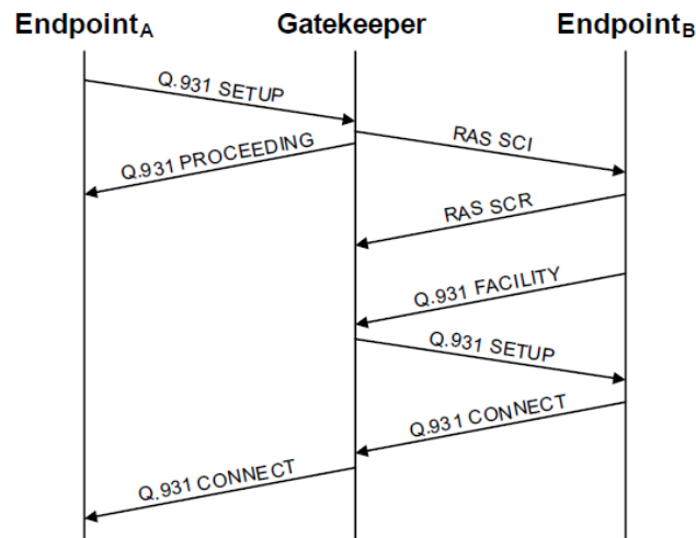
Figure 6 - H.460.18 Call Signalling Messages
