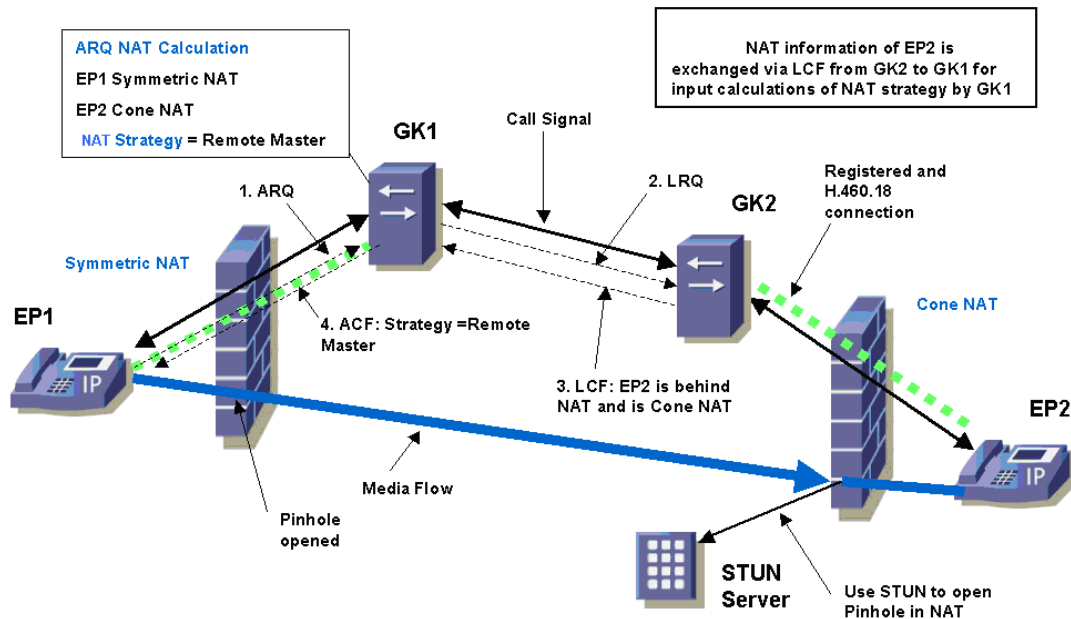
Figure 7 - Direct Media with Double NAT
