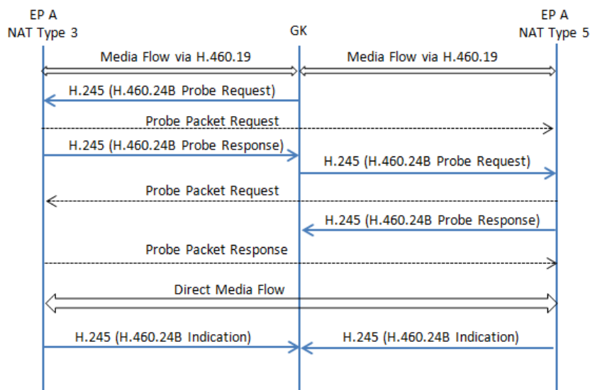
Figure 8 – H.460.24 Annex B Call Flows
